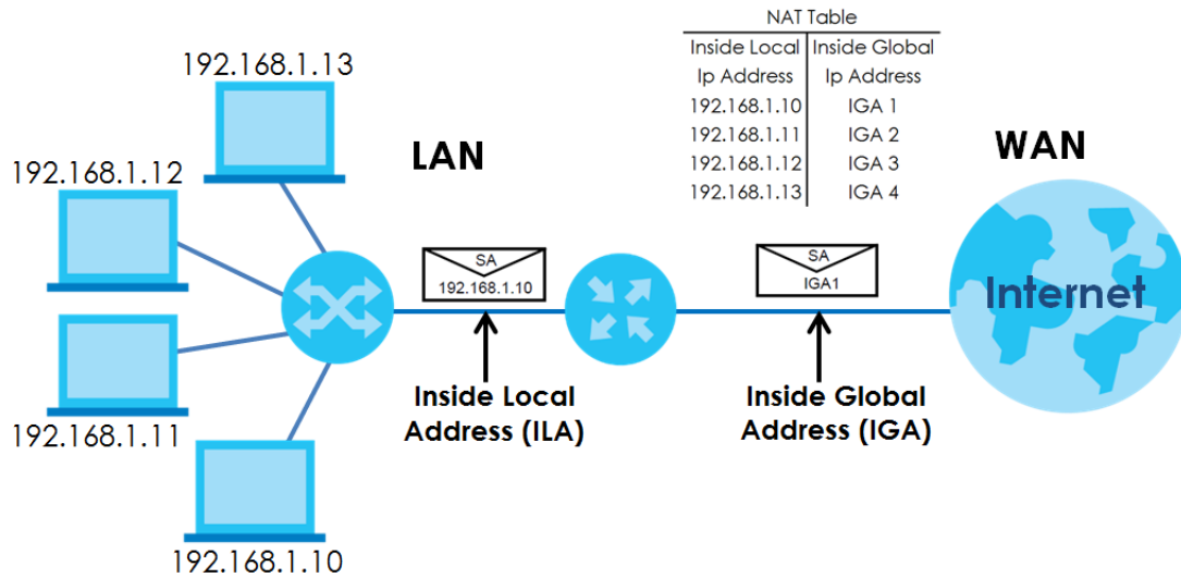
Figure 179 How NAT Works
