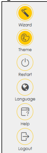
Figure 25 Side Bar
