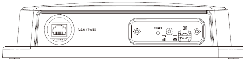
Figure 11 Bottom Panel (NR7102)
