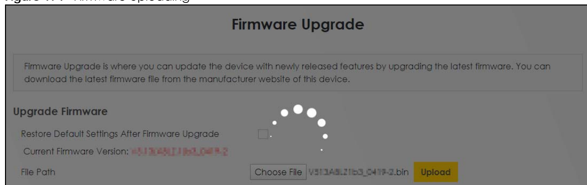
Figure 174 Firmware Uploading
