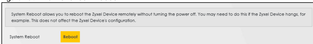
Figure 184 Maintenance > Reboot
