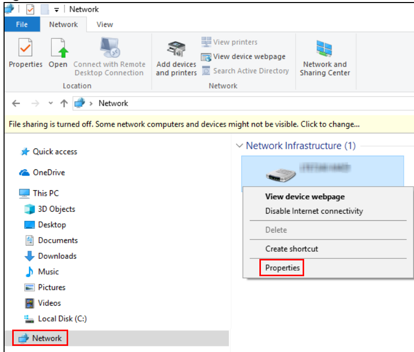
Figure 90 Network Connections
