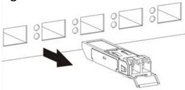
Figure 46 Transceiver Removal Example
