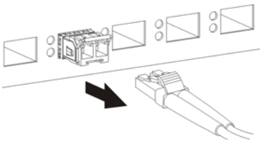
Figure 45 Opening the Transceiver's Latch Example
