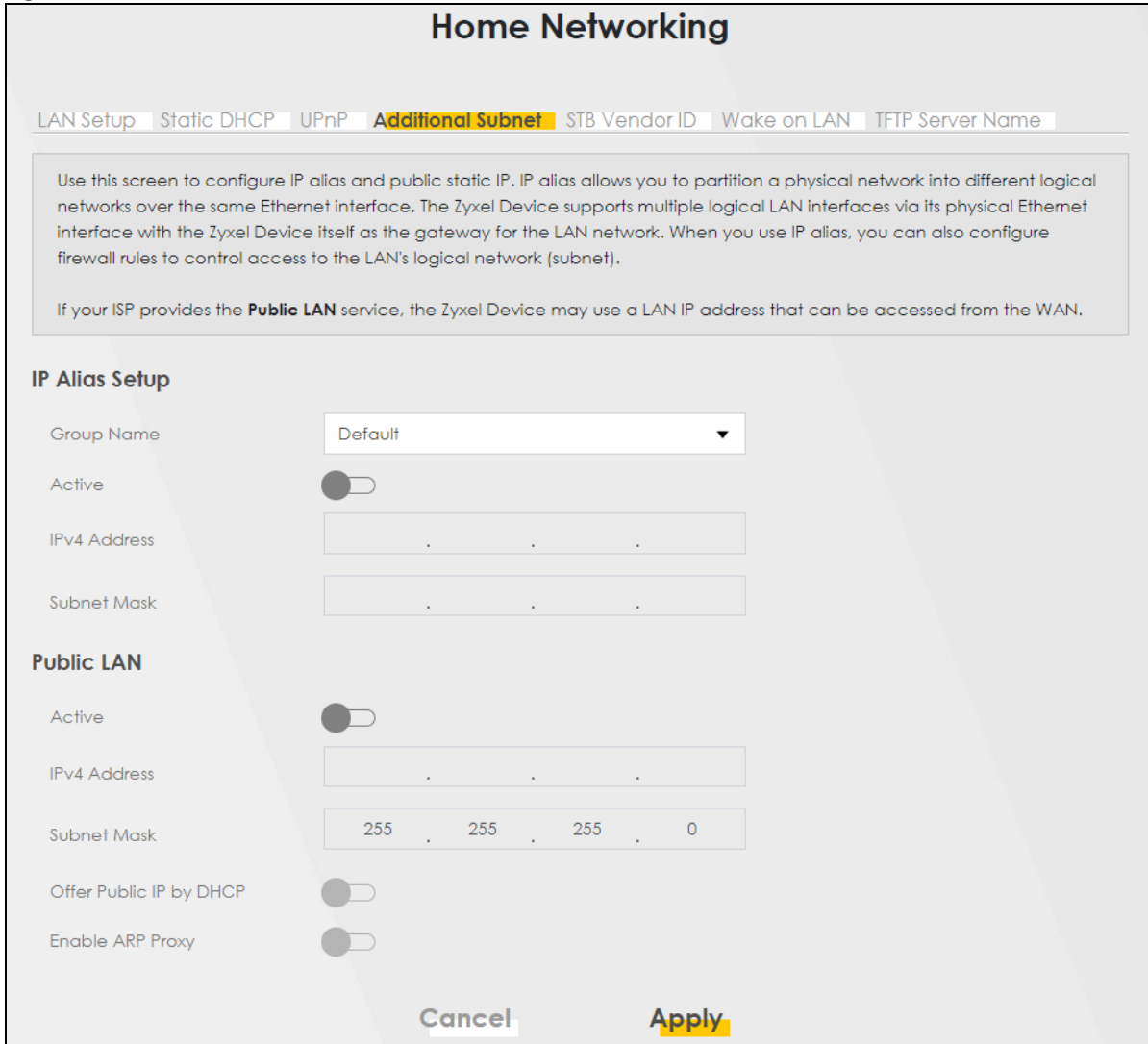
Figure 131 Network Setting > Home Networking > Additional Subnet
