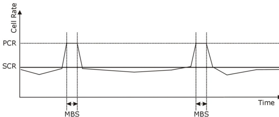
Figure 112 Example of Traffic Shaping
