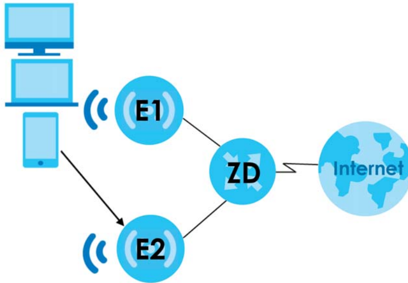
Figure 72 AP Steering Application
