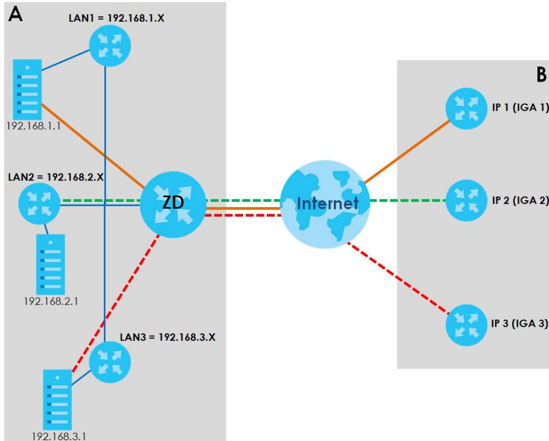
Figure 187 NAT Application With IP Alias
