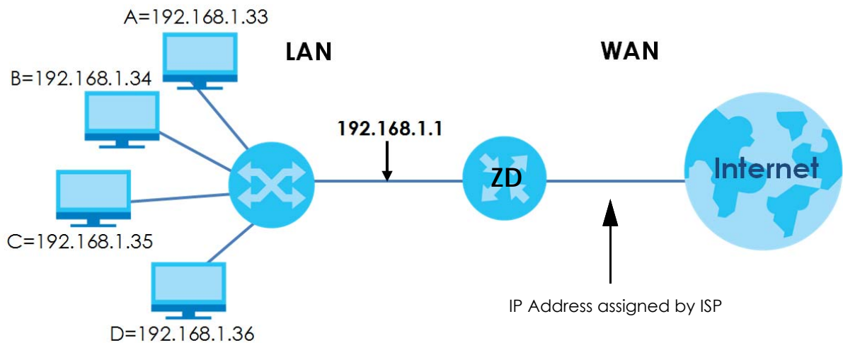
Figure 188 Multiple Servers Behind NAT Example
