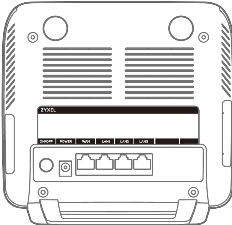
Figure 34 EX3500-T0
