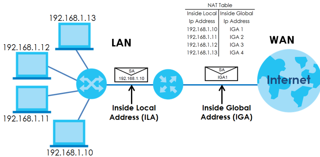
Figure 186 How NAT Works
